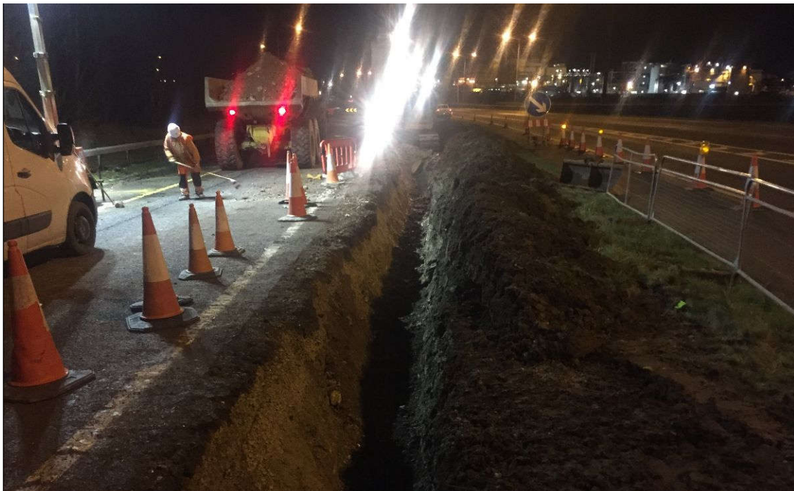
Dunkettle Interchange Upgrade: Installation of service ducting on the N25 EB off-slip road
