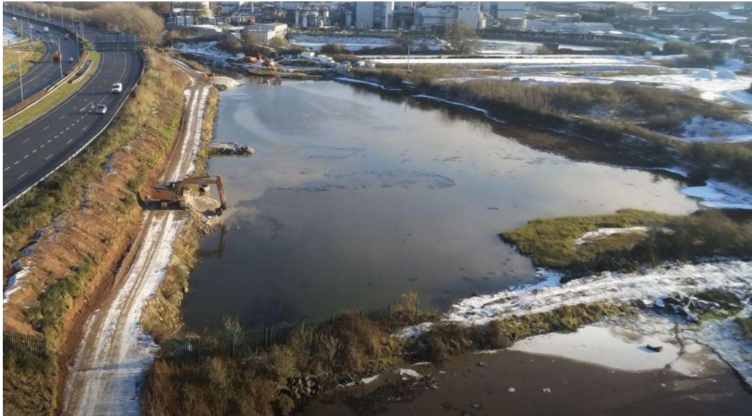
Piling platforms under construction to facilitate installation of test piles at proposed new bridge locations south of the N25
