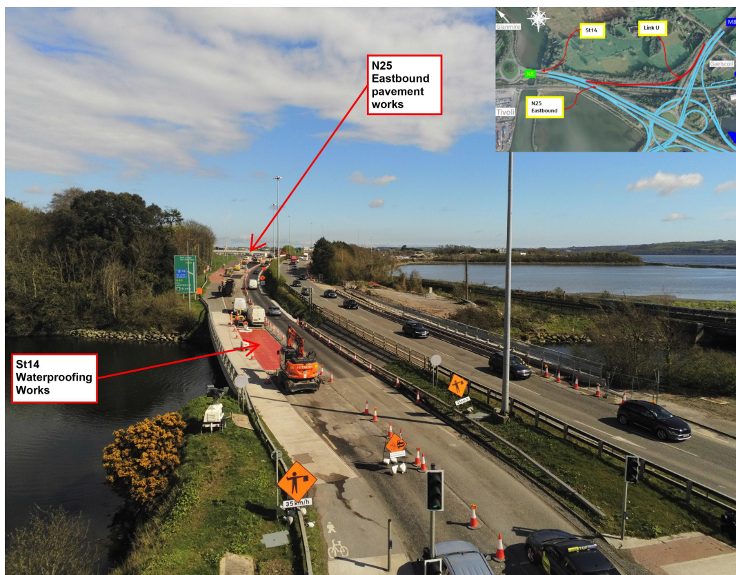
Waterproofing works at St14 on the N25 eastbound.
