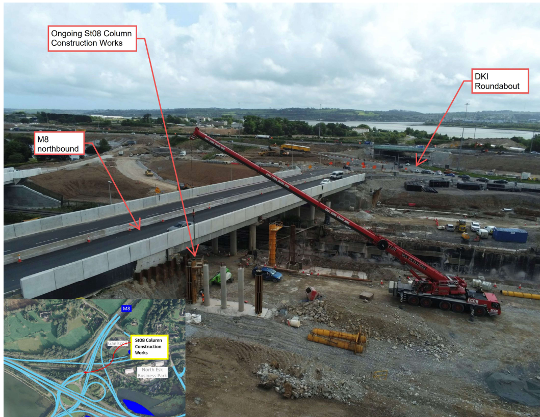
Column construction works ongoing alongside the M8 northbound.
