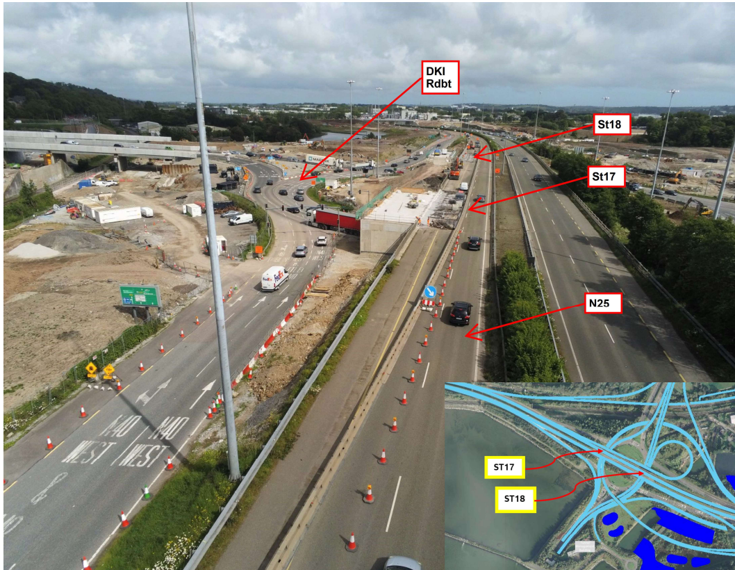
Preparatory works ongoing for waterproofing of the existing structures on the N25 eastbound.
