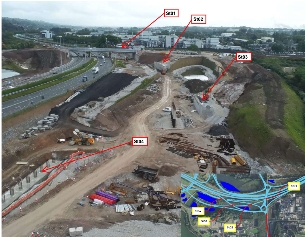
Works ongoing for Structures alongside the N25 westbound.
