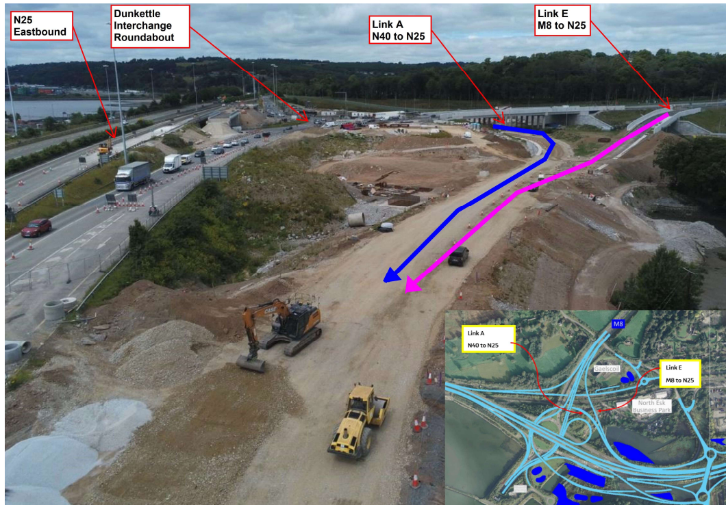
Earthworks ongoing on site alongside the N25 eastbound.
