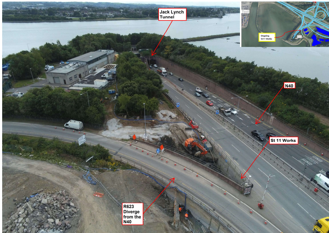
Excavation works ongoing at Structure St11 on the approach to the Jack Lynch Tunnel.
