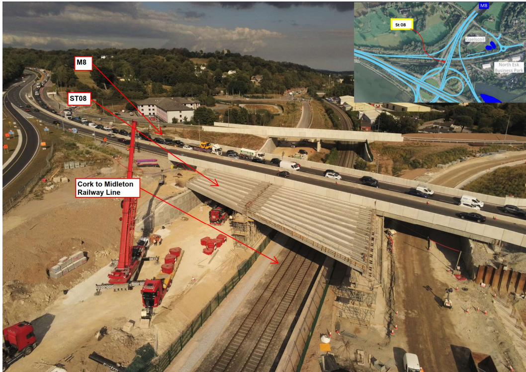
Precast concrete beams in place at ST08 west alongside the M8 northbound.
