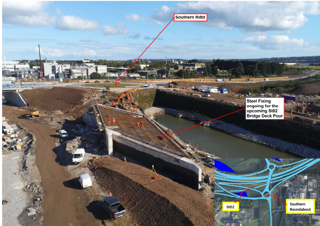
Steel Fixing works ongoing at Structure St02.
