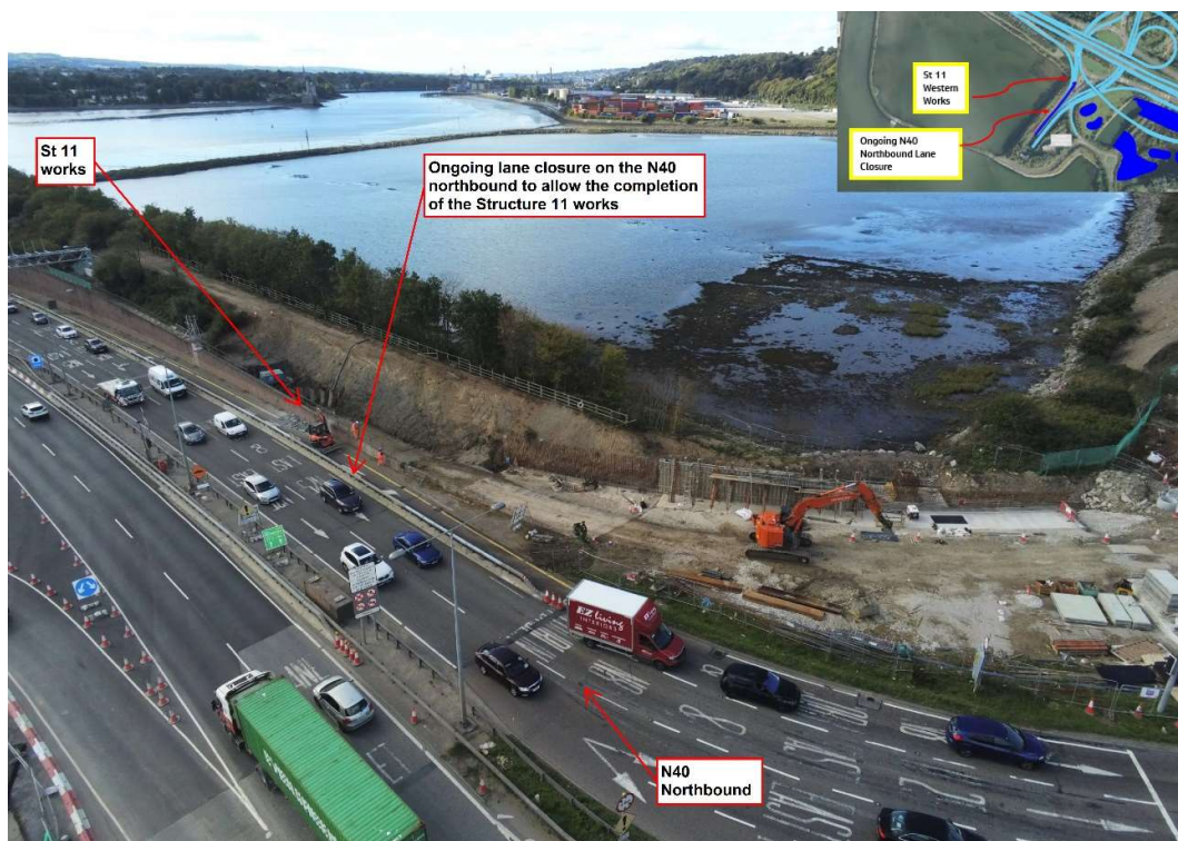
Ongoing works on the N40 northbound approach to the DKI Roundabout.
