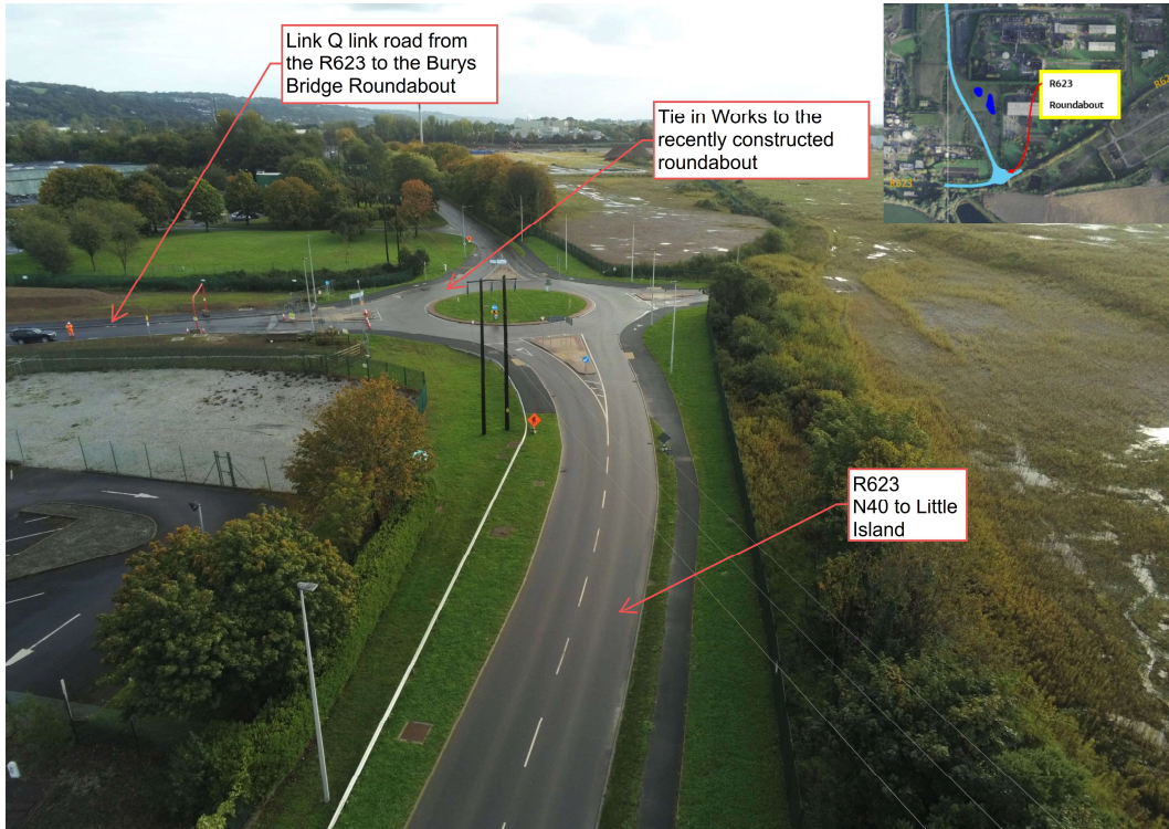
Pavement works area on the R623 Little Island access from the N40 southbound
