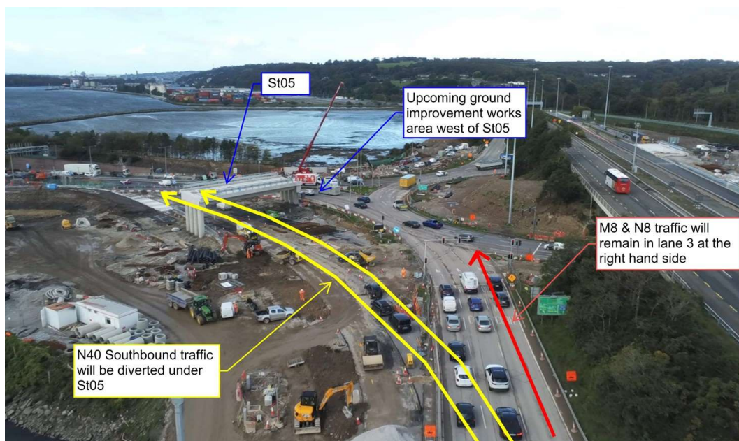
Upcoming traffic realignment on the N25 westbound diverge approach to the Dunkettle Interchange Roundabout.
