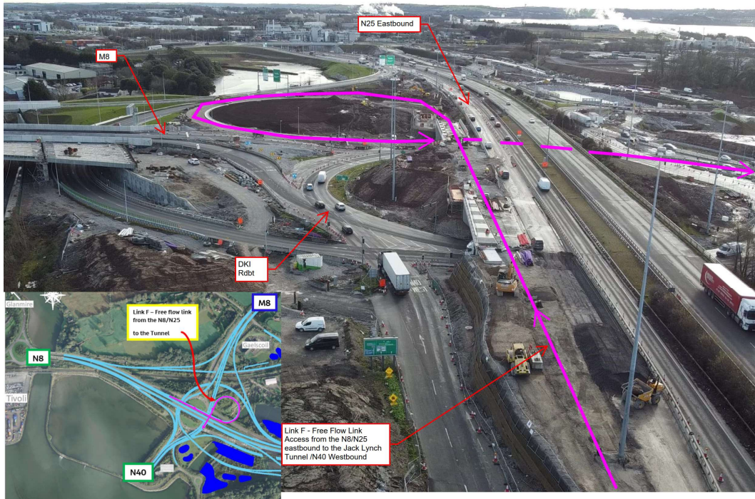
Embankment construction being progressed at Link F alongside the N25 eastbound.
