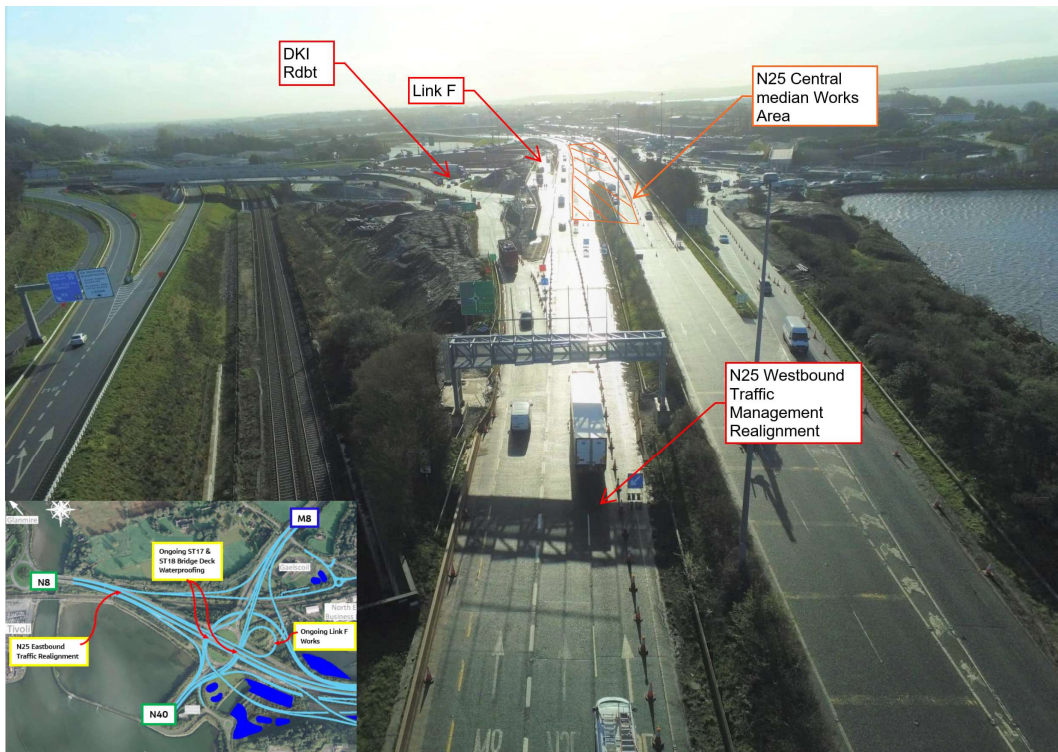
Works ongoing alongside the recently realigned N25 eastbound alongside Link F.
