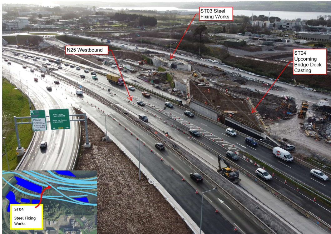
Steel Fixing works ongoing at Structure ST04 alongside the N25 westbound.
