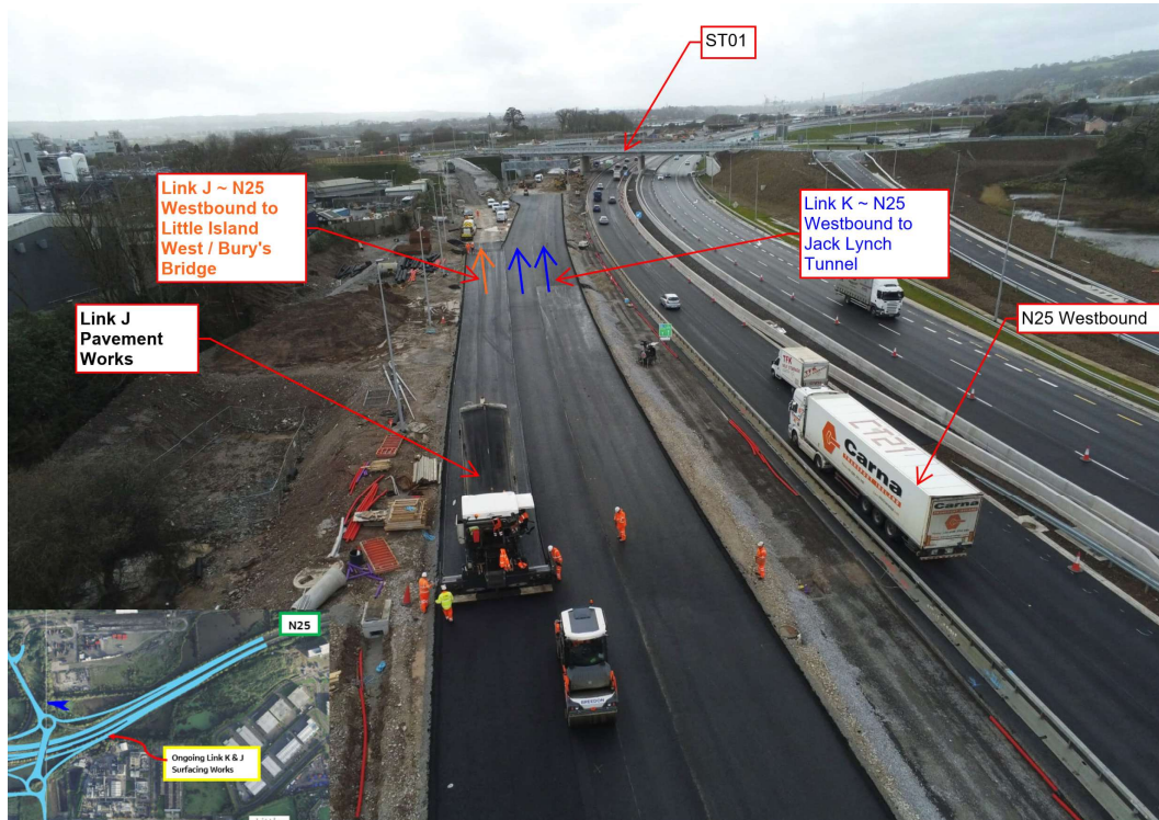
Pavement works ongoing at Link K & J alongside the N25 westbound.
