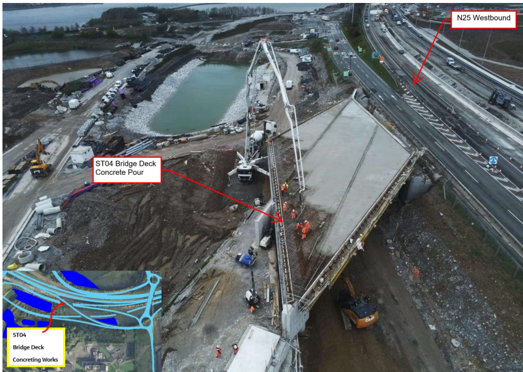
Works ongoing on site for the casting of the Structure ST04 bridge deck alongside the N25 westbound.
