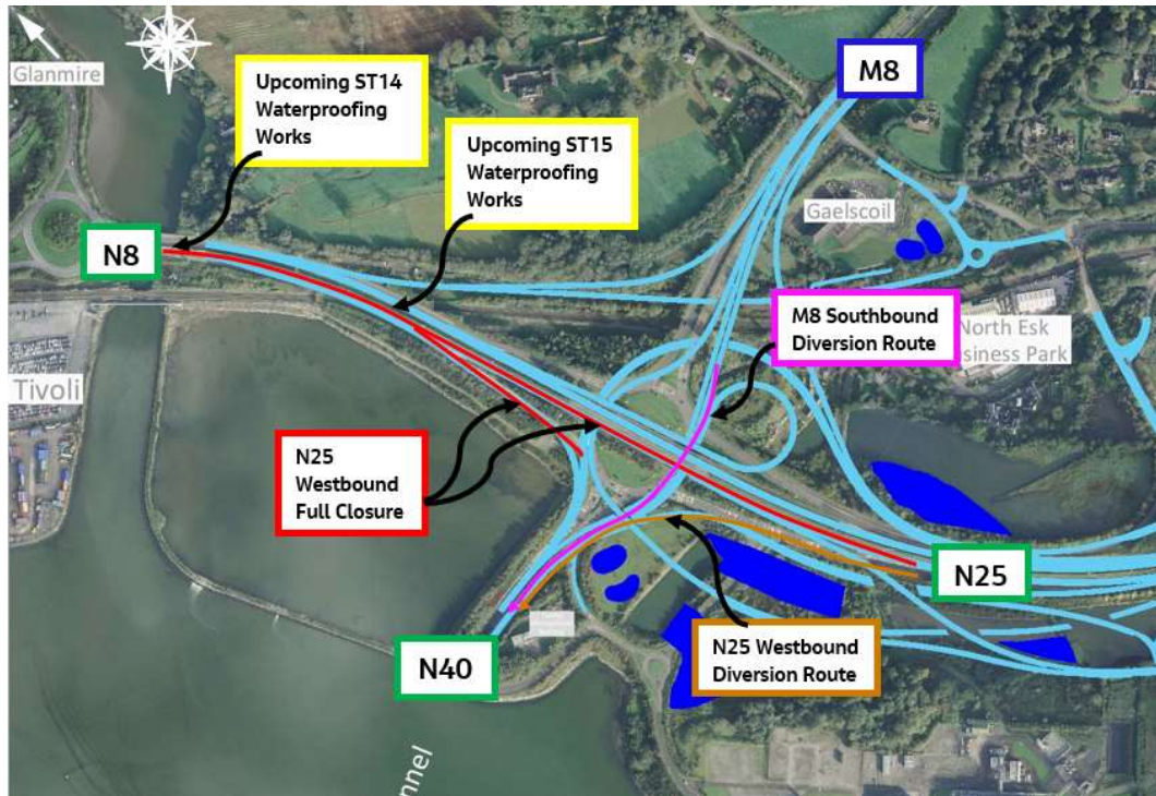
Waterproofing Works Location at Structures ST14 & ST15 on the N25 Westbound between the DKI Roundabout and the Glanmire Roundabout.
