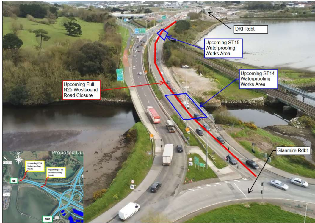
Upcoming Waterproofing Works at Structure ST14 on the N25 eastbound.
