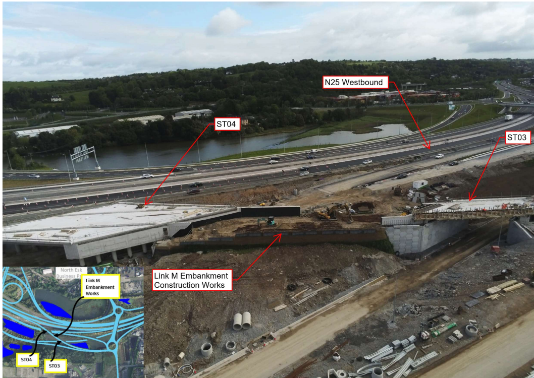
Embankment construction works ongoing between ST03 & ST04.
