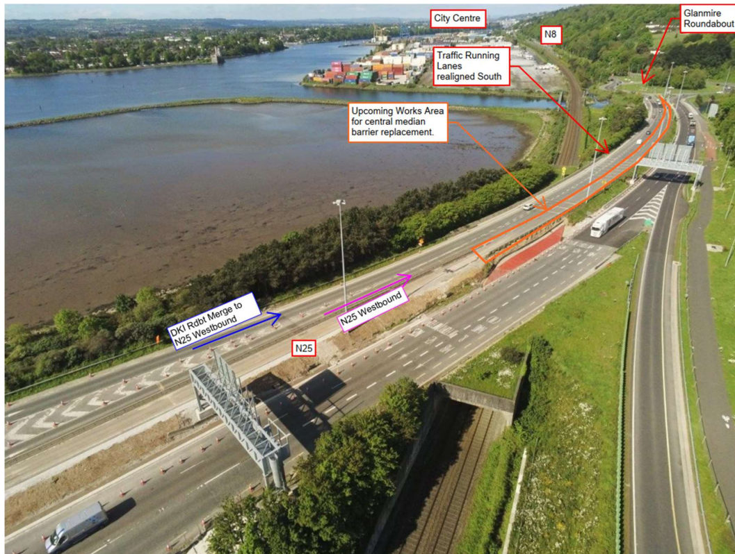
The realigned running lanes on the N25 Westbound approach to the Glanmire Roundabout.
