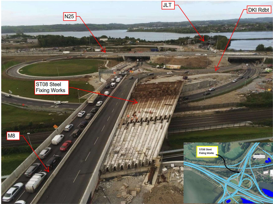
Steel Fixing works ongoing at Structure ST08.
