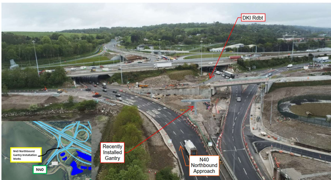
Gantry installation works ongoing on site.
