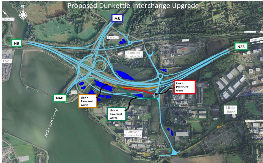
Upcoming surfacing works on Links L, K & M.
