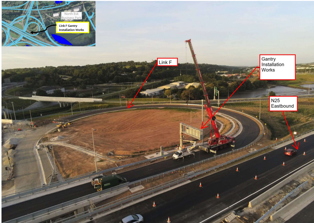
Link F Gantry Installation under night-time working.
