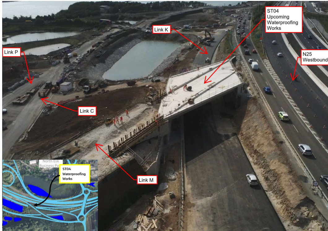
Upcoming Structure ST04 waterproofing works.
