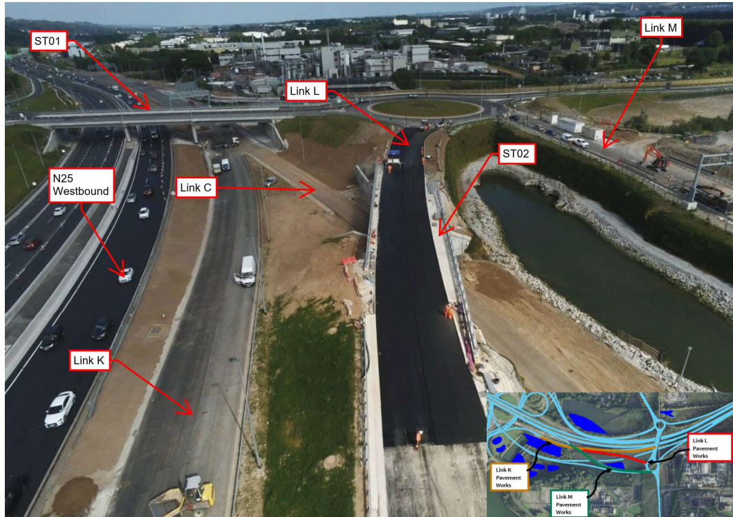
Upcoming surfacing works on Links L, K & M.
