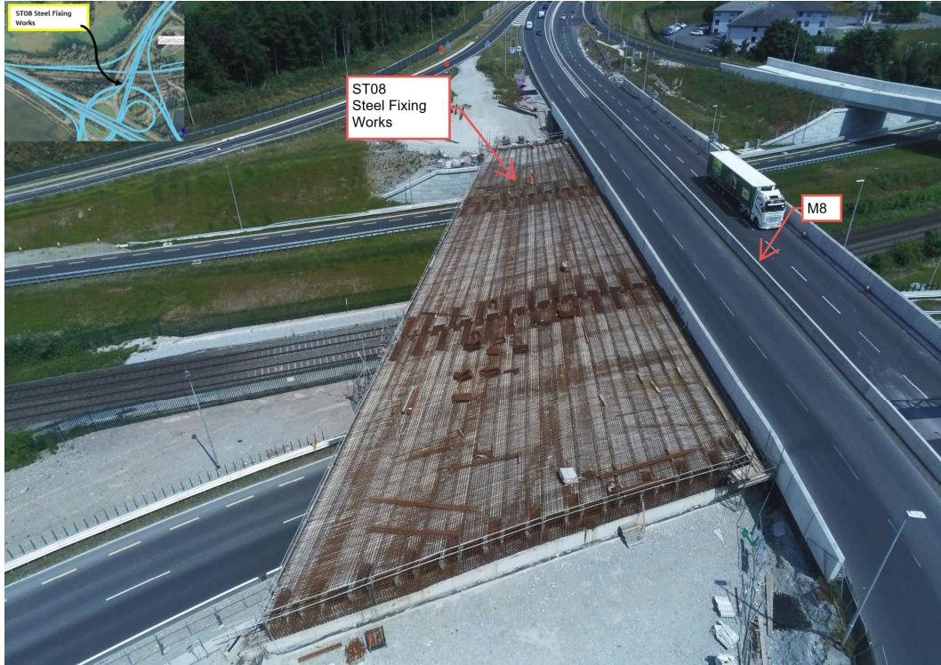
Ongoing steel fixing works at Structure ST08.
