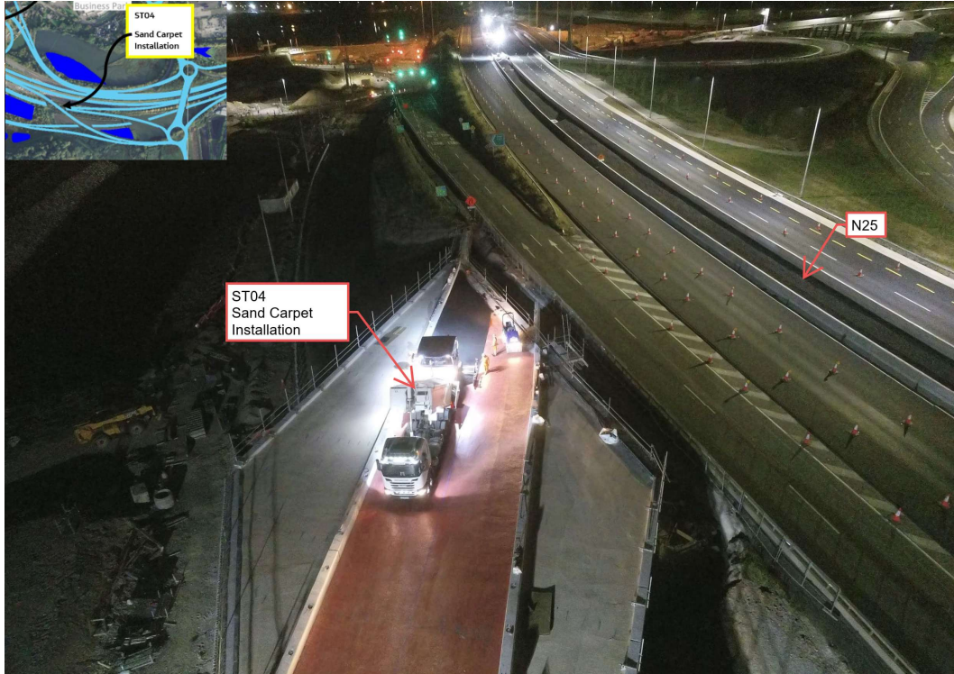
Sand Carpet Installation at Structure ST04.
