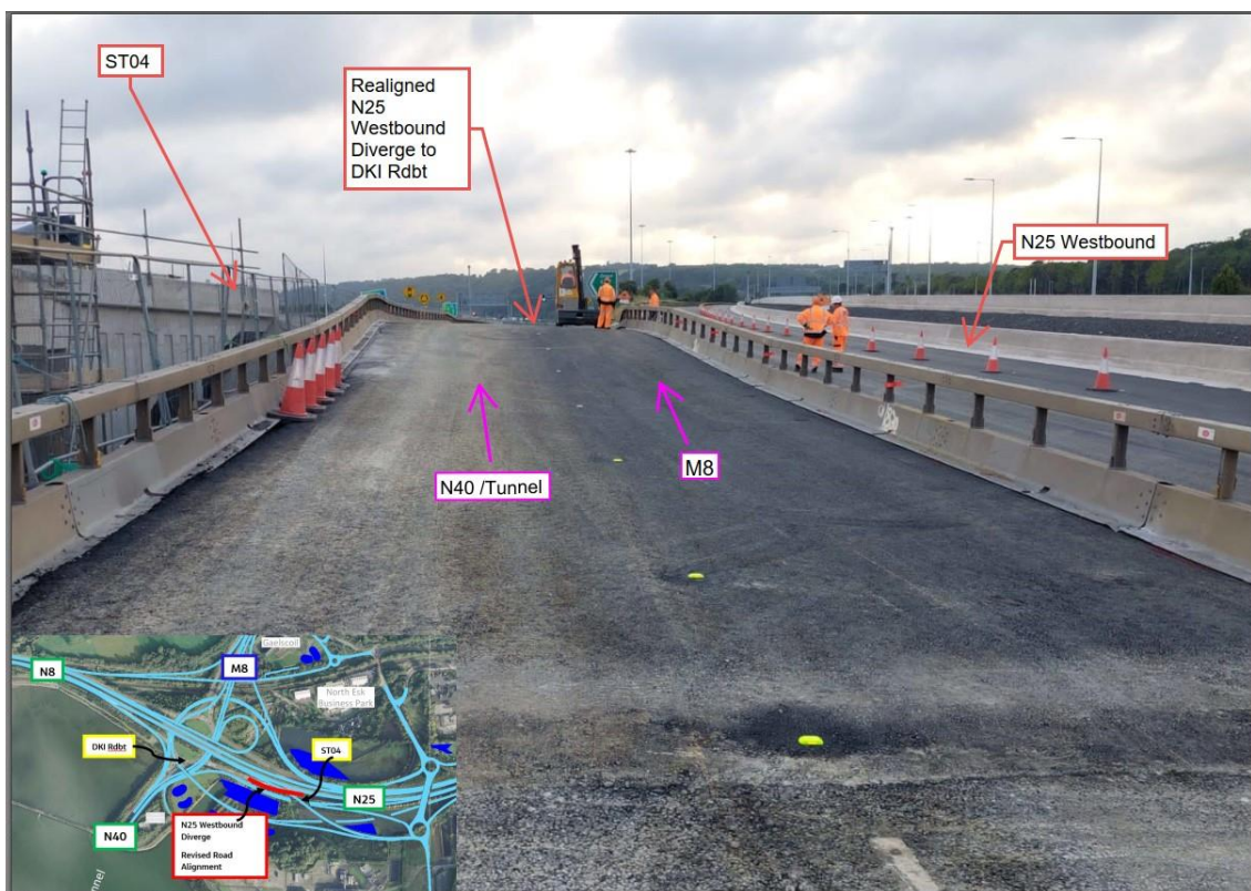
Revised Road alignment on the N25 Westbound Diverge approach to the Interchange Roundabout
