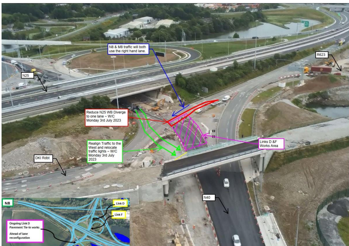
Upcoming lane reconfiguration on the M8 Southbound approach to the Tunnel.
