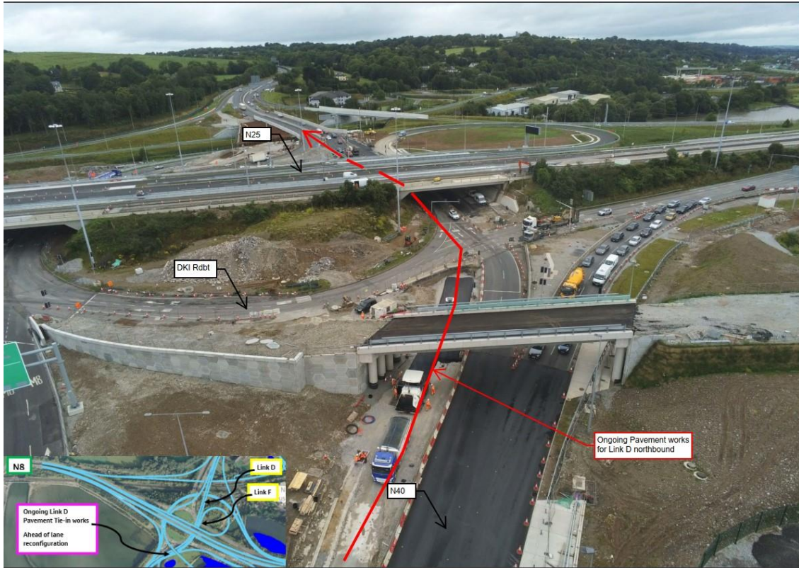
Surfacing works being progressed in the vicinity of the DK1 Rdbt. for Link D Northbound.
