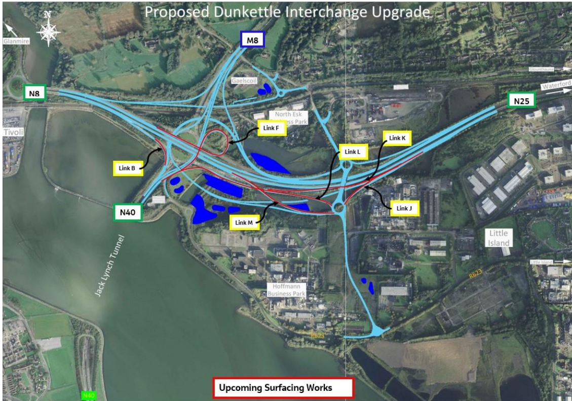
Location of the upcoming surfacing works on site.
