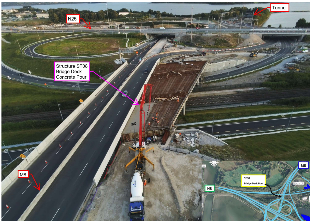
Bridge Deck Concrete Pour on the Northern span of Structure ST08
