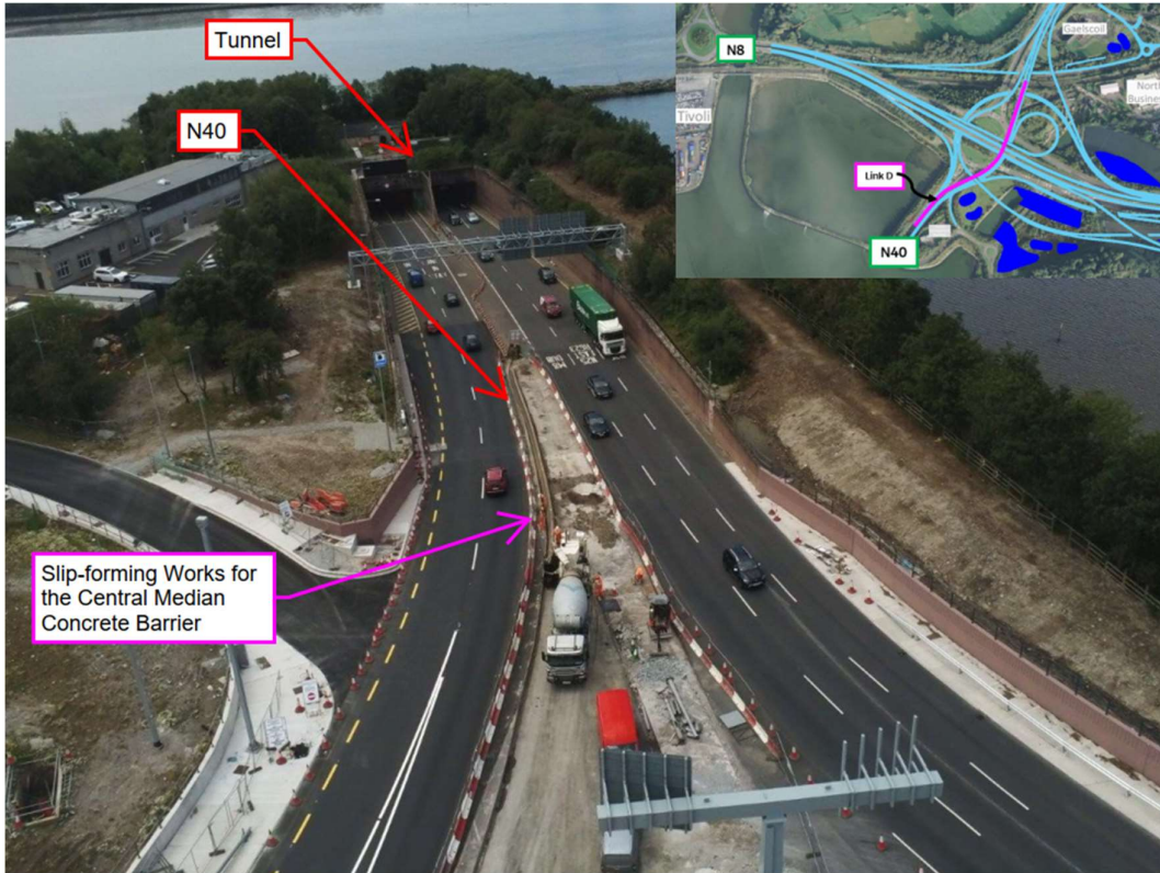
Slipform concreting works being undertaken alongside the N40 southbound
