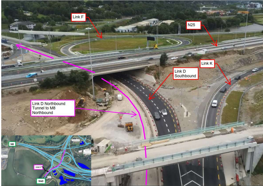
Works ongoing at Link D northbound in the area of the old Dunkettle Interchange Roundabout
