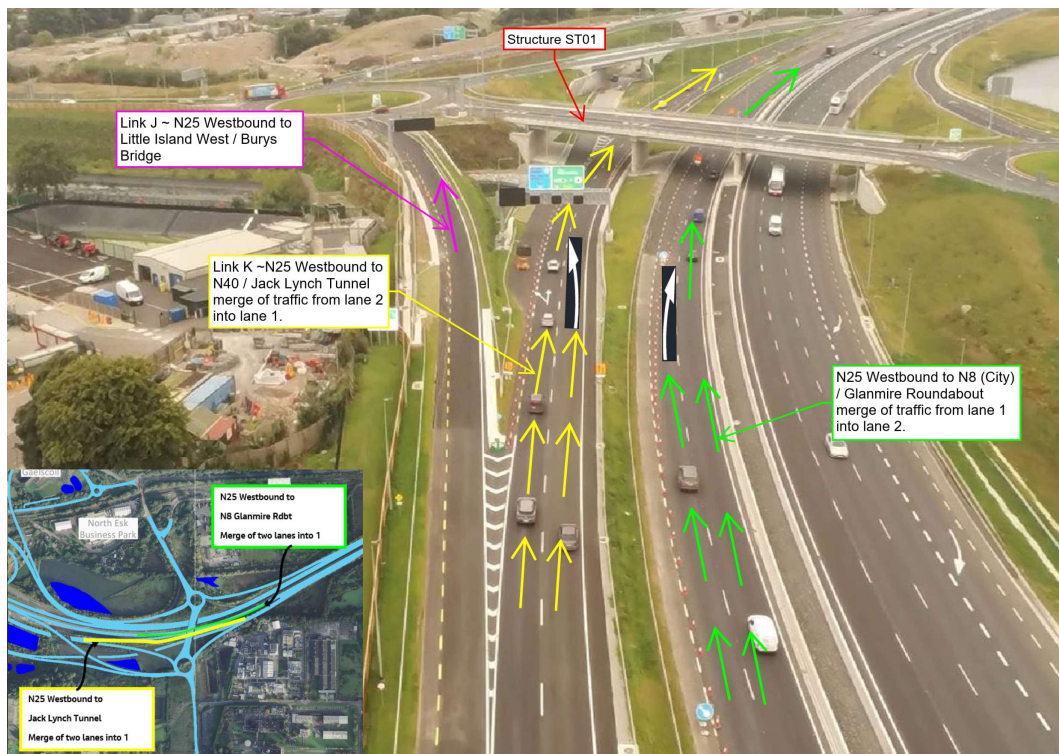
Current Traffic Management layout on the N25 Westbound.
