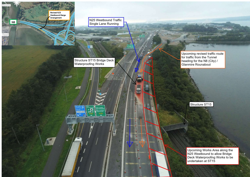
Upcoming revised traffic management layout on the N25 westbound in the vicinity of Structure ST15.
