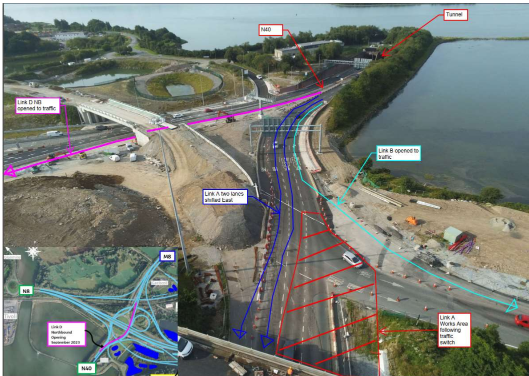
Upcoming traffic switch in the vicinity of the N40 northbound approach to the old Interchange Roundabout for M8 northbound traffic.
