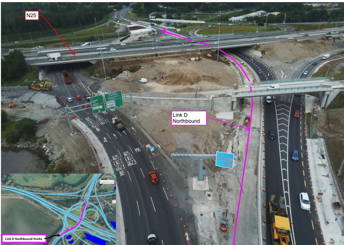
Ongoing preparatory works for the upcoming Link D northbound pavement works.
