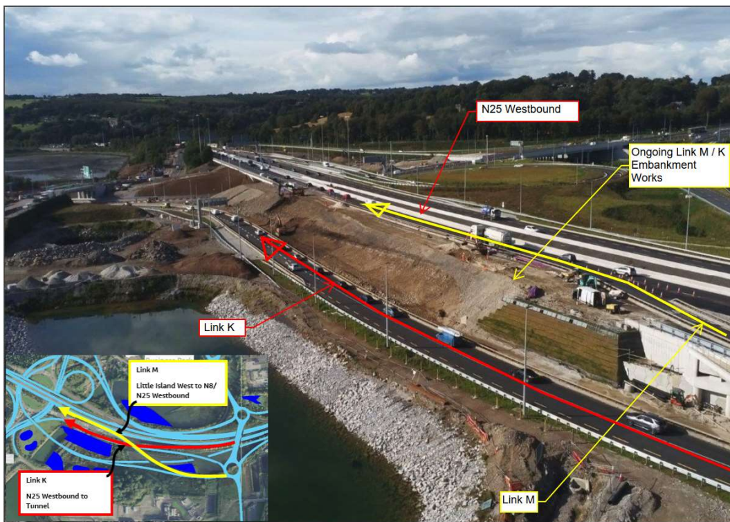
Link K & Link M Works ongoing alongside the N25 Westbound
