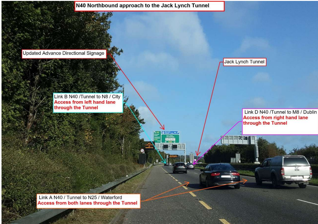
New lane configuration in place directly south of the Jack Lynch Tunnel on the N40 northbound
