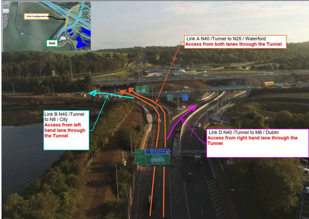
New lane configuration in place directly north of the Jack Lynch Tunnel
