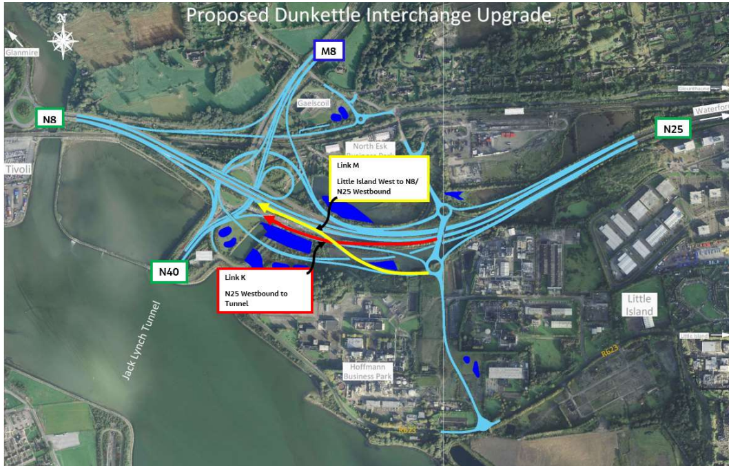
Link K & Link M Ongoing Works Location
