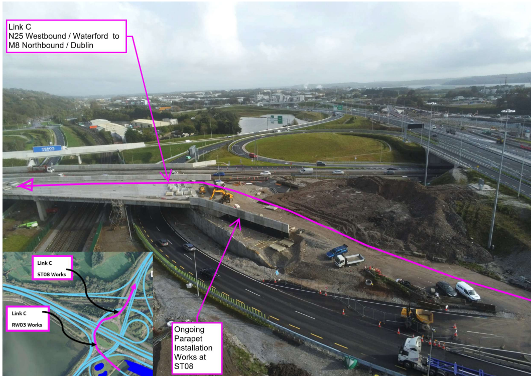
Parapet walls installed at Structure ST08 west for Link C
