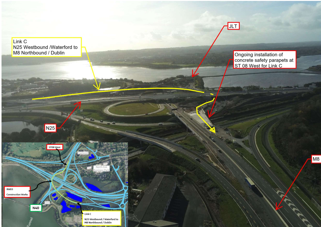
Installation of parapets at Structure ST08 (West)
