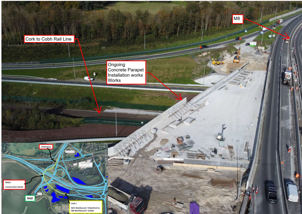
Installation of the concrete parapet railing over the Cork to Cobh railway line undertaken recently.
