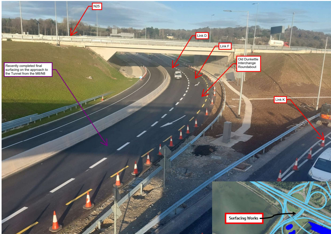
Surfacing Works ongoing on site in the vicinity of the old Interchange Roundabout
