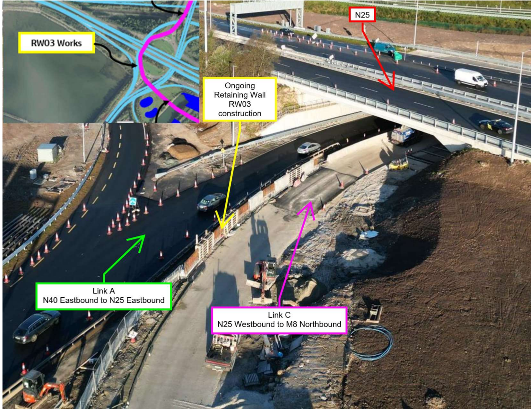
Ongoing Retaining Wall, RW03, construction at Link C
