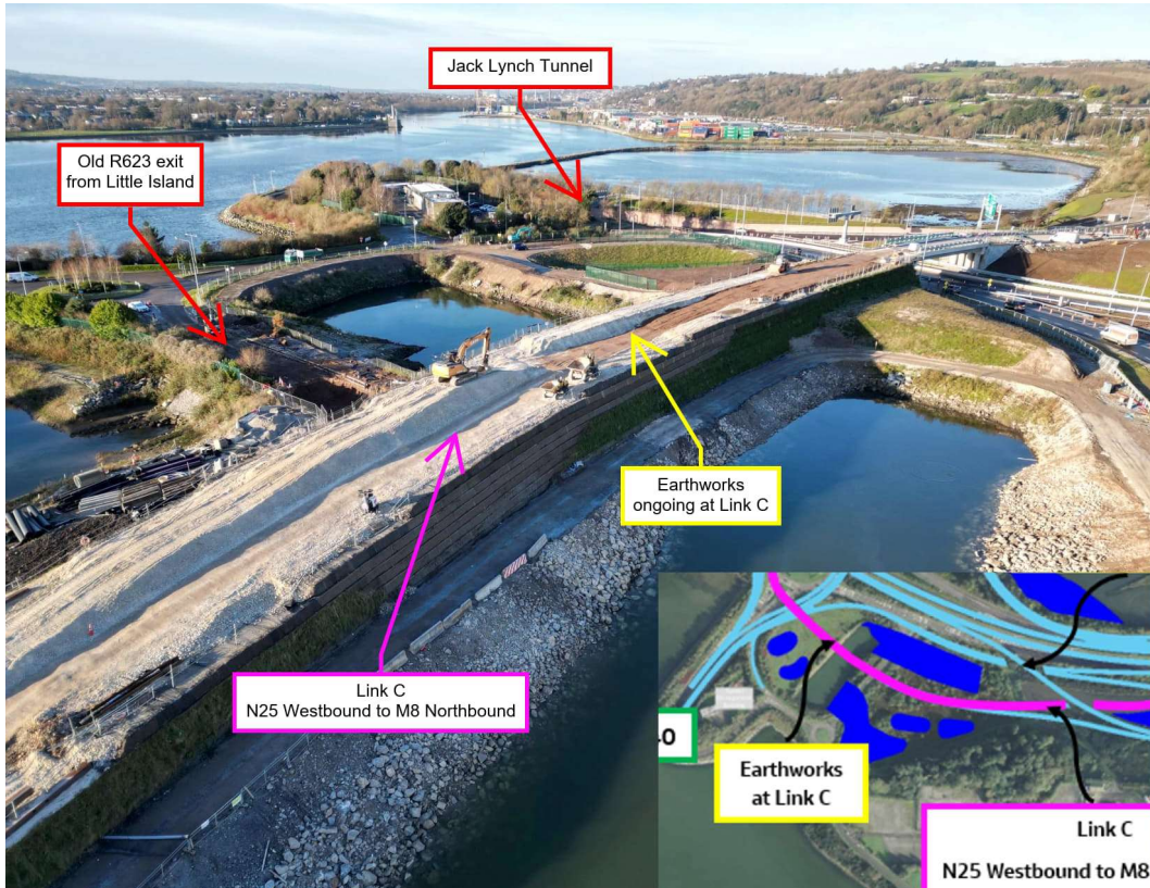
Link C Earthworks at the crossing point with the old R623.
