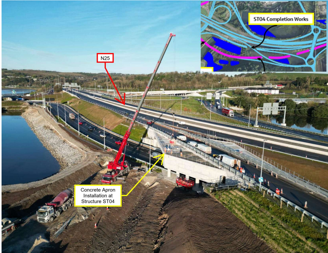
Completion works at Structure ST04
