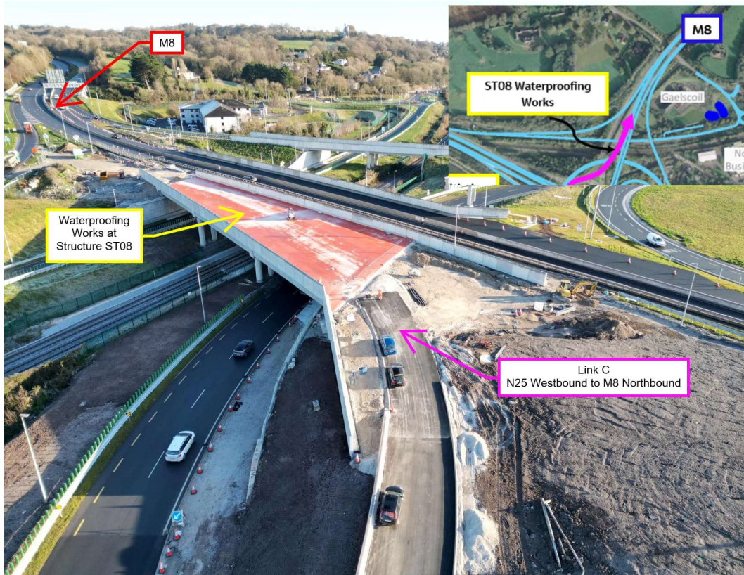
Completion of waterproofing at Structure ST08
