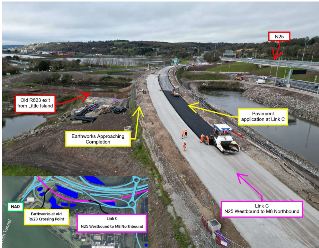
R623 / Link C crossing point – Earthworks approaching completion and ongoing Pavement works
