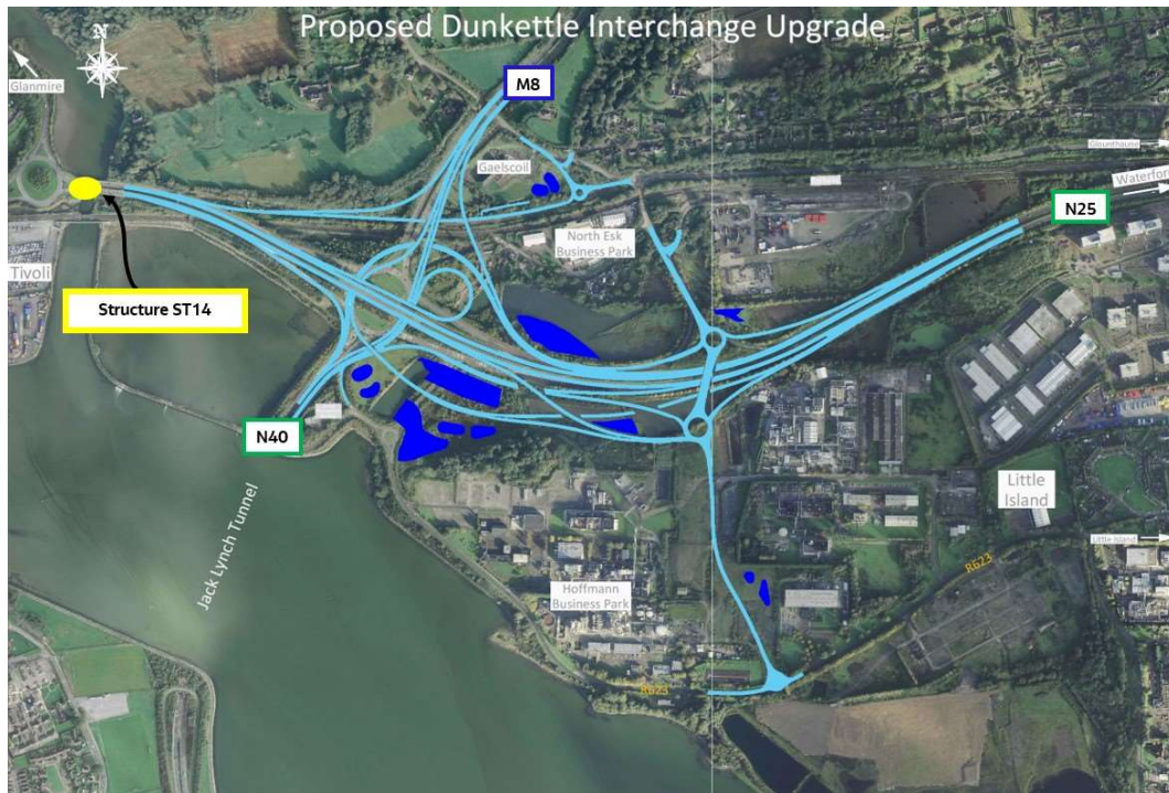
Layout Plan highlighting the location of Structure ST14
